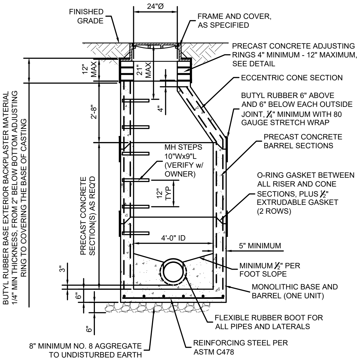
STANDARD SANITARY SEWER MANHOLE SCALE: NONE
